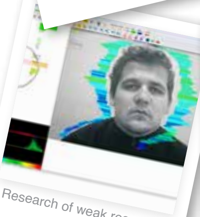
Artificial Intelligence
