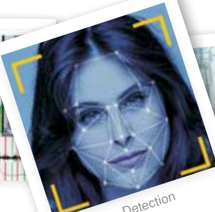
Lie Detection
