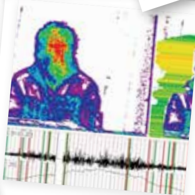
Lie Detection
